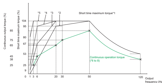
50Hz torque reference
