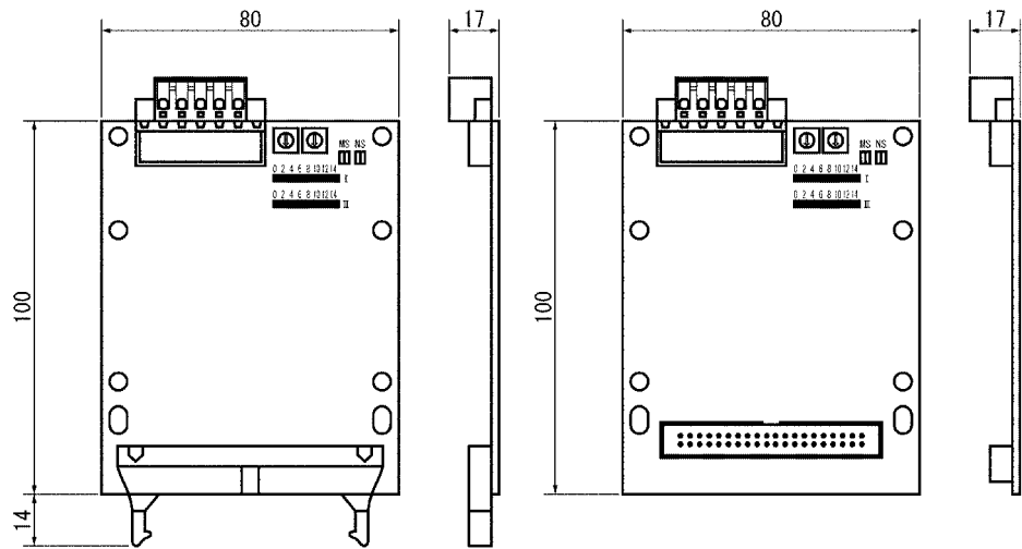
DRT2-MD32B (NPN)/DRT2-MD32B-1 (PNP) DRT2-MD32BV (NPN)/DRT2-MD32BV-1 (PNP)
