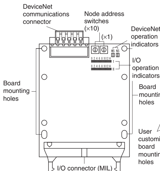
DRT2-ID32B (NPN)/DRT2-ID32B-1 (PNP)
