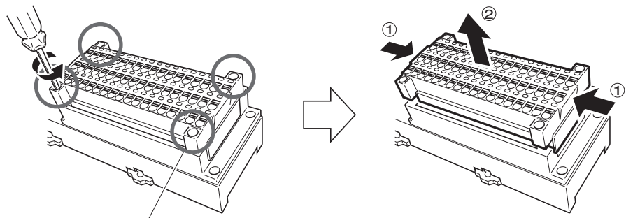
Four 2.6x6 standard screws
