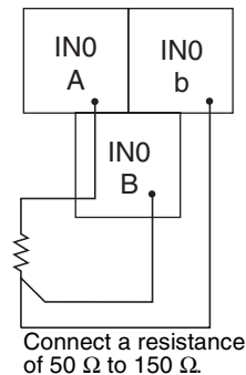
DRT2-TS04P Platinum-resistance thermometer input
