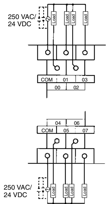
CPM1A-8ER
